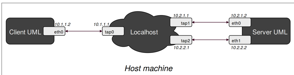
Figure 5.6. Network scenario, client one interface and server two interfaces (IPv4)
