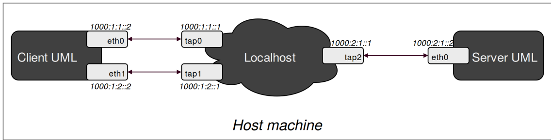
Figure 5.7. Network scenario, client two interfaces and server one interface (IPv6)
