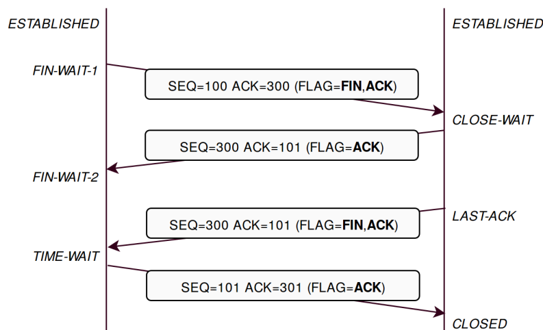
Figure 2.3. Normal TCP connection termination procedure
