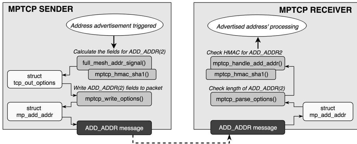
Figure 5.5. ADD_ADDR(2) operational flow in the MPTCP network stack
