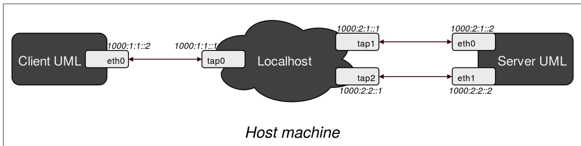
Figure 5.8. Network scenario, client one interface and server two interfaces (IPv6)
