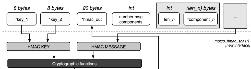
Figure 5.4. New API for mptcp_hmac_sha1()
