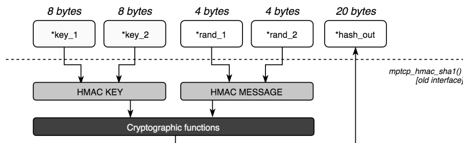
Figure 5.3. Old API for mptcp_hmac_sha1() [46]
