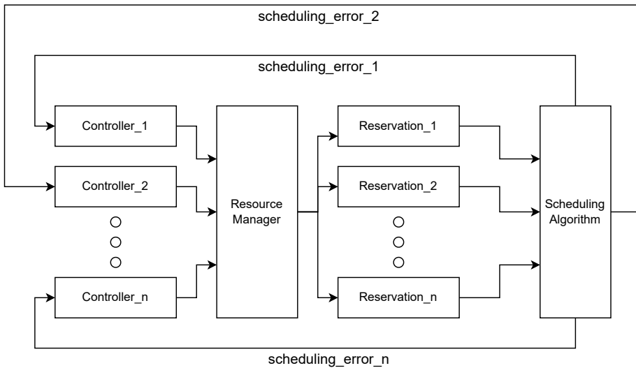
Fig. 2.1. Adaptive Reservation Architecture from [18, 19].
