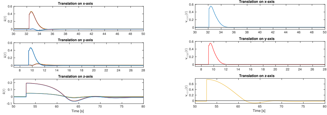
(a) Feature Error. Each curve represents a feature component error (x and y in the image plane). (b) IBVS Velocity Module. The curves in blue, red and yellow represent the desired velocity along the x , y and z axis.
