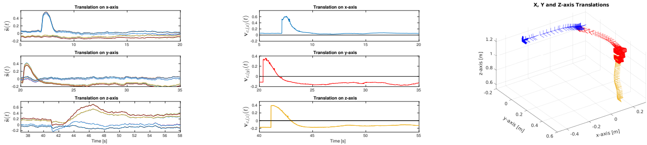
(a) Feature Error for x , y and z translations, top to bottom. Each curve represents a feature component error (x and y in the image plane). (b) IBVS Velocity Module. The curves in blue, red and yellow represent the desired velocity along the x , y and z axis, respectively. (c) 3D Trajectory of the UAV. Blue, red and yellow represent the translations on x , y and z respectively.
