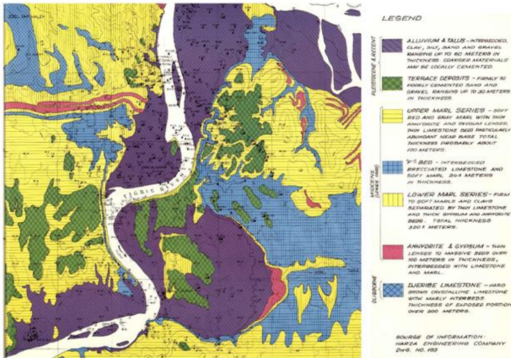
Figure 8: Geologic map of Mosul Dam site area [36].
