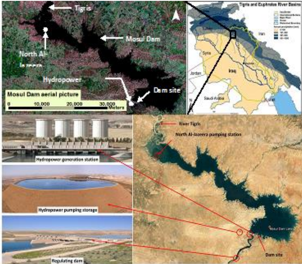
Figure 4: Location of Mosul Dam with main facilities.
