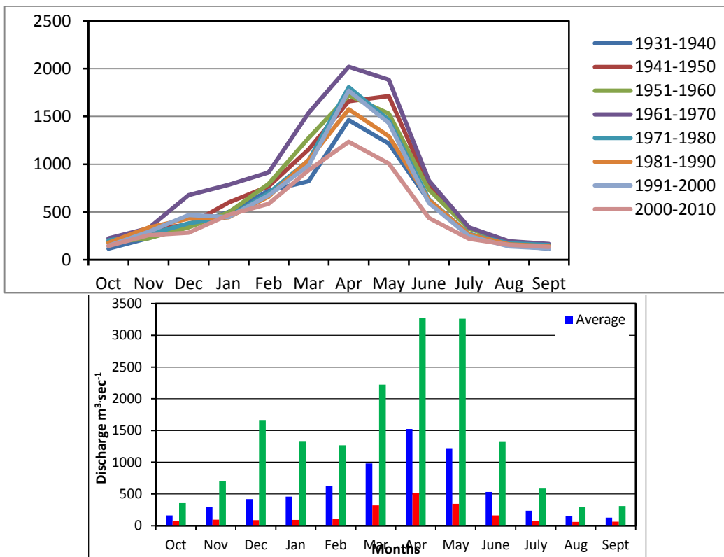
Figure 2: Monthly (mean, minimum and maximum) inflows of Tigris River at dam site (1931-2013).
