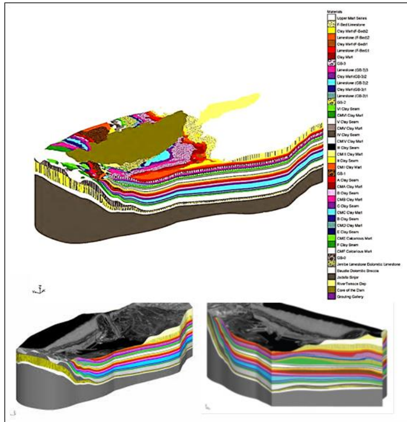
Figure 11: Three dimensional model of Mosul Dam site [24].
