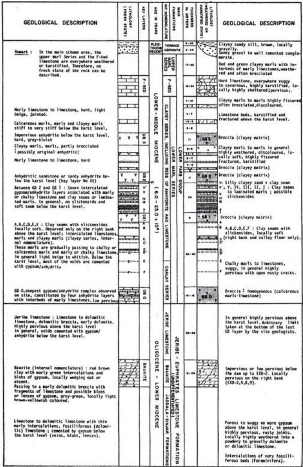
Figure 9: Lithological column of beds at Mosul Dam site [19].
