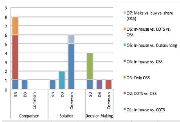
Figure 5: Dimension Coverage
