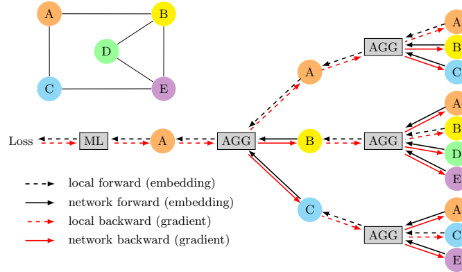
Fig. 1. Computational tree of the forward and backward passes for computing a node embedding in a 2-layer GNN. Note the large number of embeddings and gradients that would be exchanged across the network in a naive decentralized implementation.
