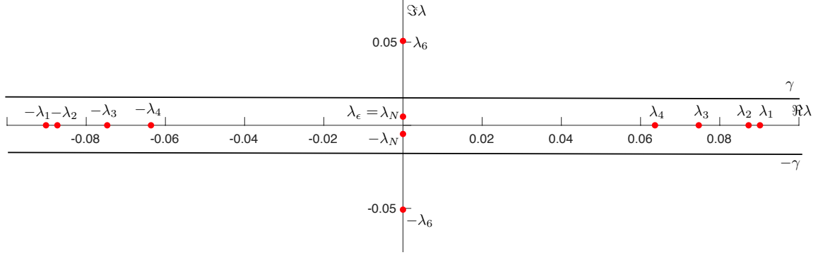
Figure 2: The values of \lambda are on the real and imaginary axis only. When the energy is close to one of the thresholds \omega_N , it is possible to choose a strip |\Im\lambda| \leq \gamma_N such that all real and only two imaginary values of \lambda are within the strip (indicated). For example when L = 80.33 and \omega = \omega_5 - \epsilon ( \omega_5 = 0.0912 and \epsilon = 0.0001 ), then all the possible values of \lambda are indicated with red dots, only real values are enumerated: \pm\lambda_1, \pm\lambda_2, \dots, \pm\lambda_4 ( N = 5 ) and the imaginary values of \lambda are indicated by \pm\lambda_\epsilon . For the sake of the proof of Proposition (2), we indicate \lambda_N ( \lambda_N = \lambda_5 in our case and \lambda_N = \lambda_\epsilon as \omega is slightly less and close to the threshold) and \lambda_{N+1} = \lambda_6 .
