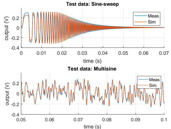
Fig. 3. The first part of the test data: the measured is in blue, and the simulated is in red. Observe how the simulated output follows closely the test data.
