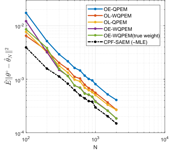
Fig. 1. The MSE of six different estimators approximated using 1000 Monte Carlo realizations.
