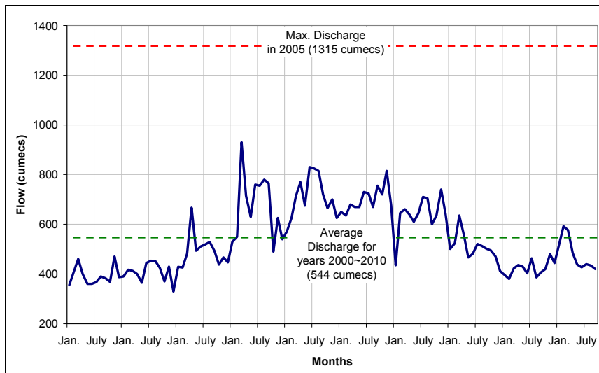
Figure 2: Recorded Tigris River flow at Sarai Baghdad station for the period 2000-2010. Data source: [Shahrabaly, 2008]
