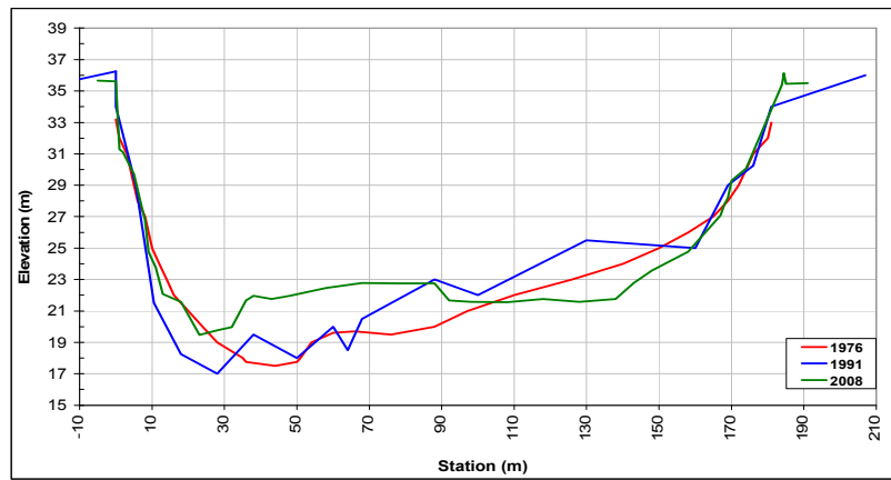
Figure 6: Changing in geometry shape of Sarai Baghdad gauging station.
