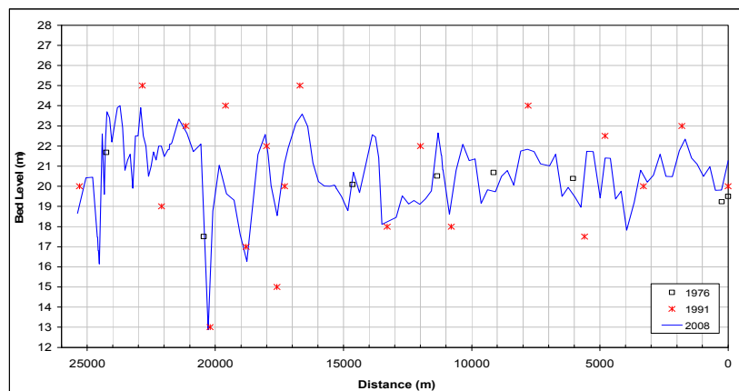
Figure 5: Tigris River bed elevations during 1976, 1991 and 2008.
