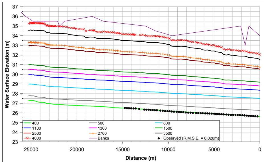
Figure 9: Computed water surface elevations for different discharge in Tigris and Diyala Rivers with discharge of 5m 3 /s with calibration data.
